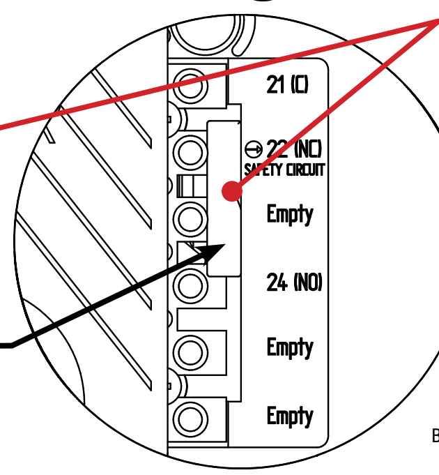
DETAIL B
