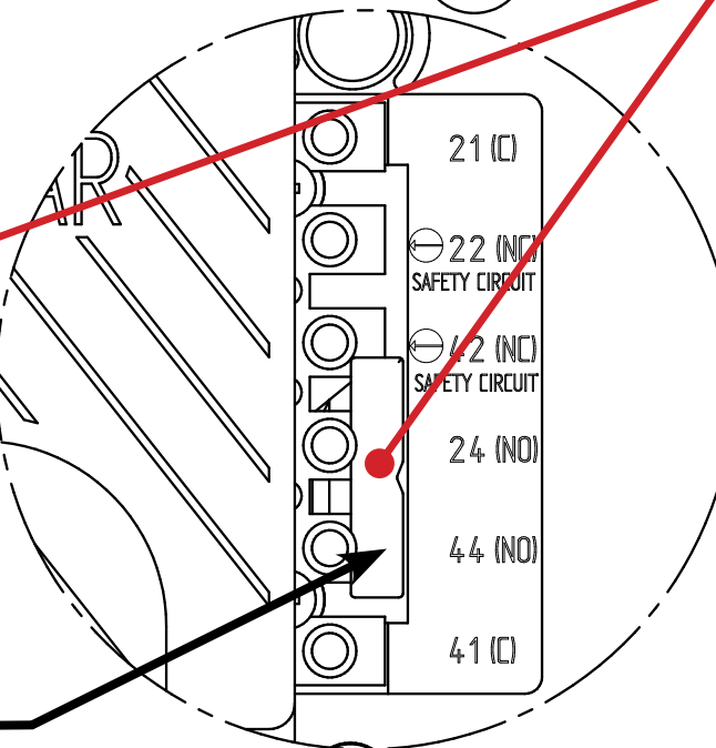
DETAIL B
