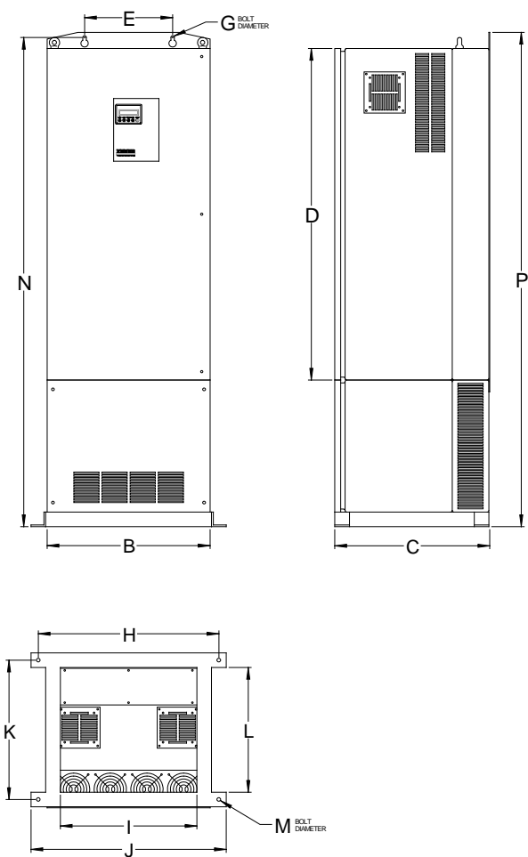
Chassis D with floor mount kit
