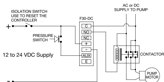
F30-DC WIRING DIAGRAM
