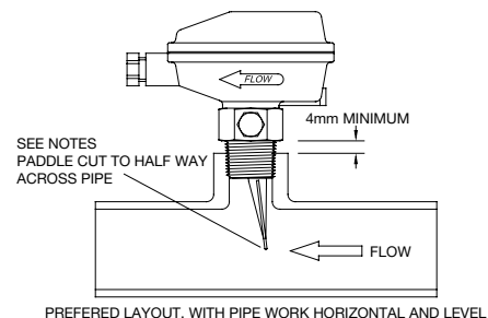
F30 MOUNTED IN A PIPE TEE
