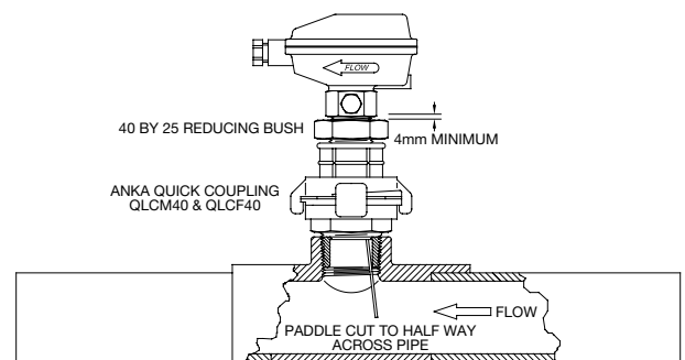
F30 MOUNTED IN A QUICK RELEASE COUPLING
