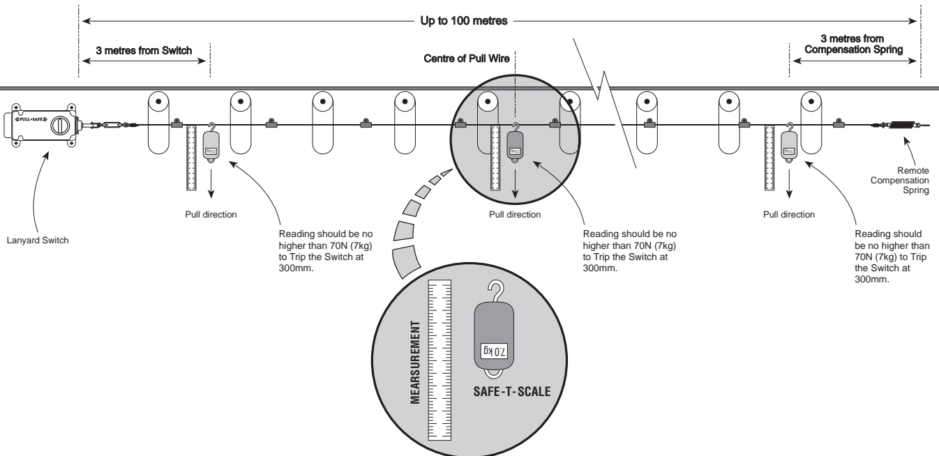
FIGURE 2 90 Degree Pull Wire Test
